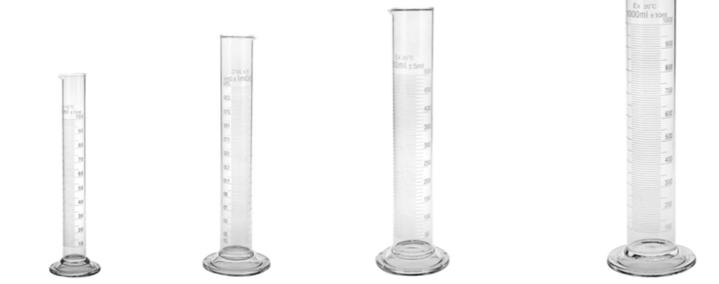
Measuring cylinder glass 100ml | Ø 3,2cm | H 25cm # 01303
